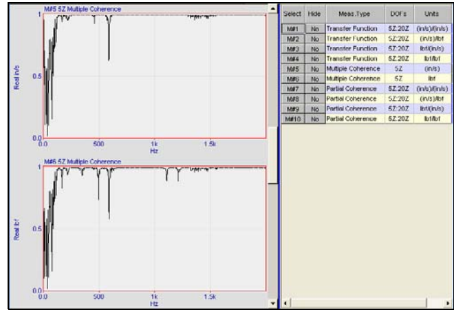
Multiple Coherences.
