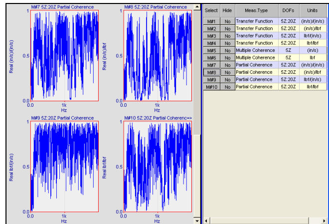
Partial Coherences.
