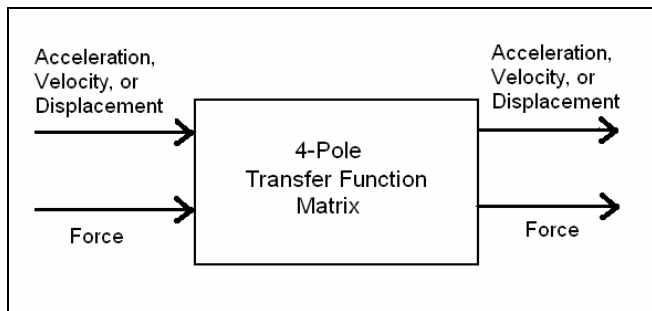
Figure 1. Block Diagram of 4-Pole Transfer Function Matrix.
