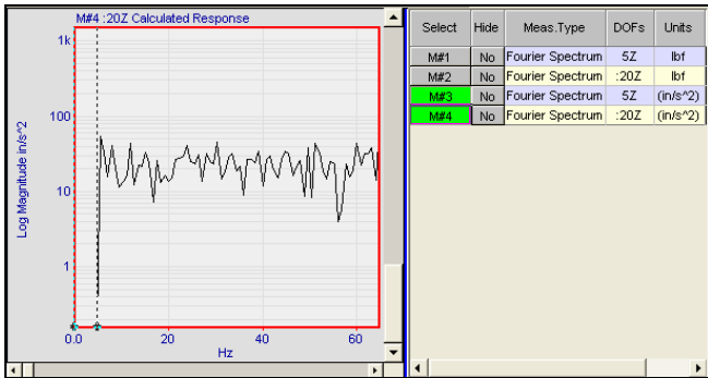
Acceleration Spectra with DC Removed.
