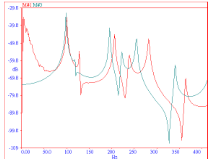
Figure 5. Synthesized Versus Measured FRF Using FEA Modes and Experimental Damping.
