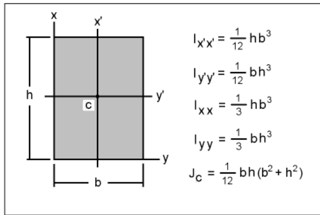
Figure 7. Rectangular Bar Cross Section.
