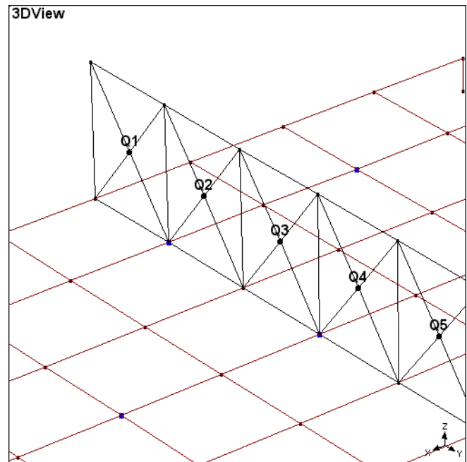
Figure 8. Zoomed View of Plate Showing Quad Elements.
