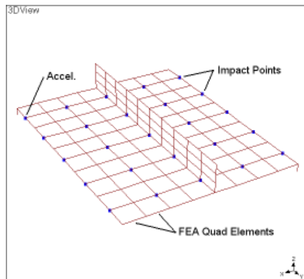
Figure 1. The Test Article.
