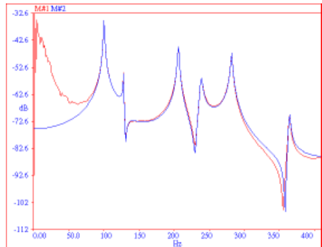
Figure 4. Synthesized Overlaid on Measured FRF (Showing First 6 Modes).
