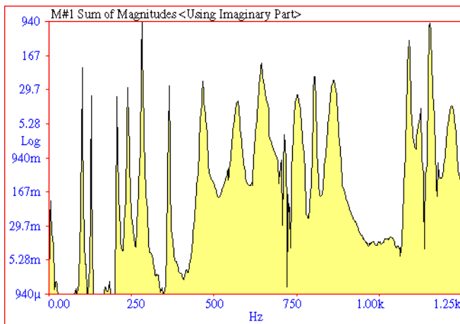
Figure 2. Sum of Magnitudes for Plate Without Rib.
