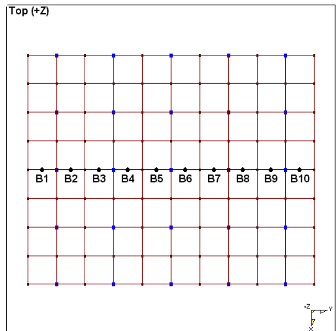
Figure 6. Top View of Plate Showing Bar Elements.
