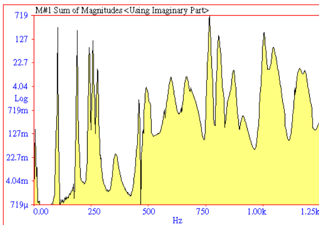
Figure 3. Sum of Magnitudes for Plate With Rib.
