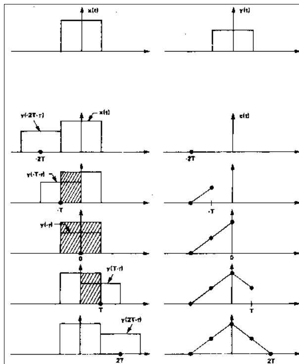
Figure 4 - Convolution of two functions.
