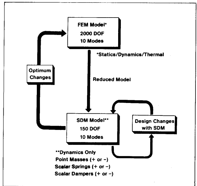
Figure 8. Relationships between FEM and SDM models.
