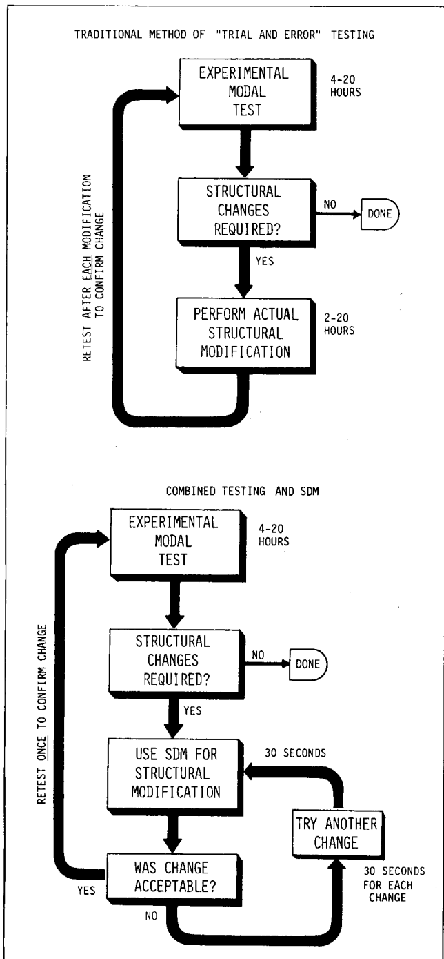
Figure 7. Procedures for troubleshooting noise and vibration problems.
