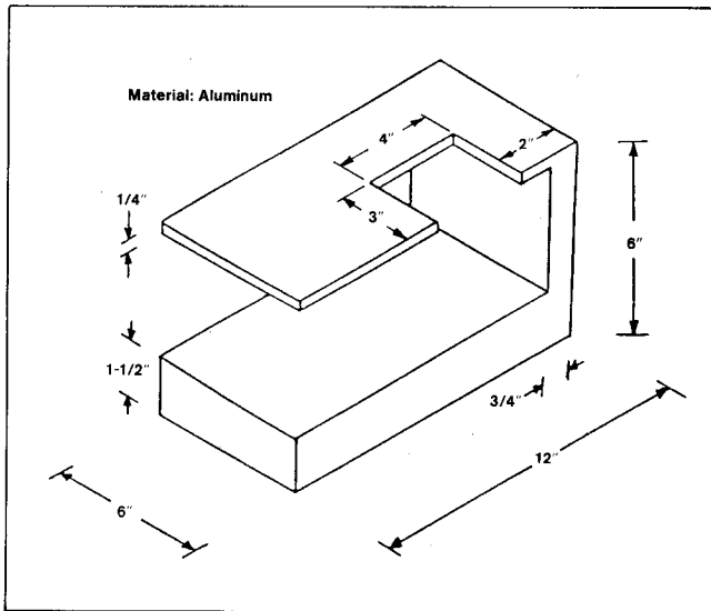
Figure 9. SDM/FESDEC test structure.
