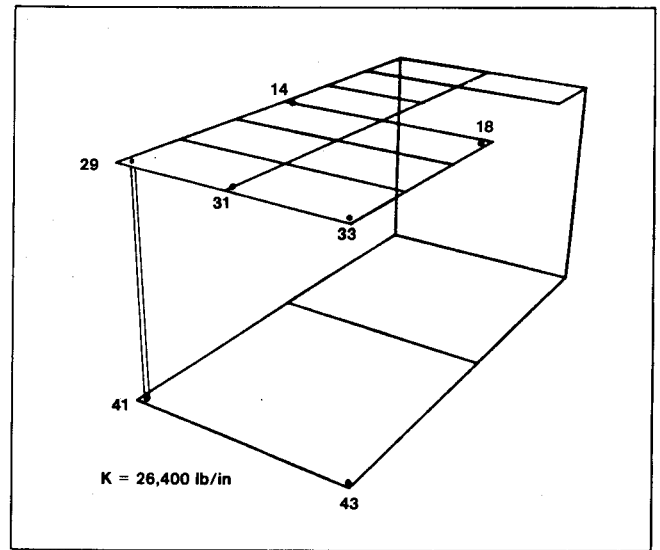
Figure 11. Modified test structure.
