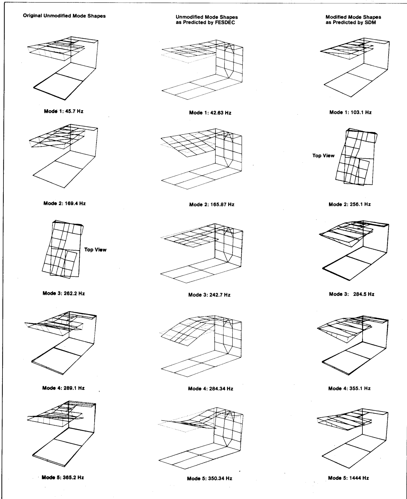
Figure 13. Comparison of mode shapes.
