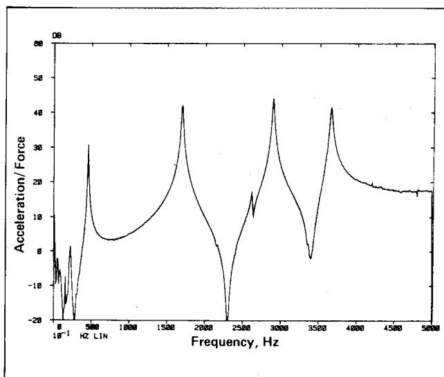
Figure 2. Frequency response measurement to identify structural resonances.
