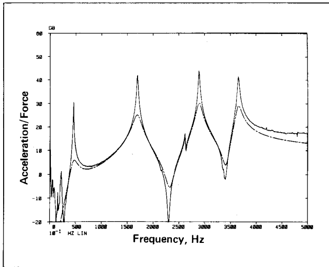
Figure 3. The effect of adding damping to reduce the dynamic response of a structure at resonance.
