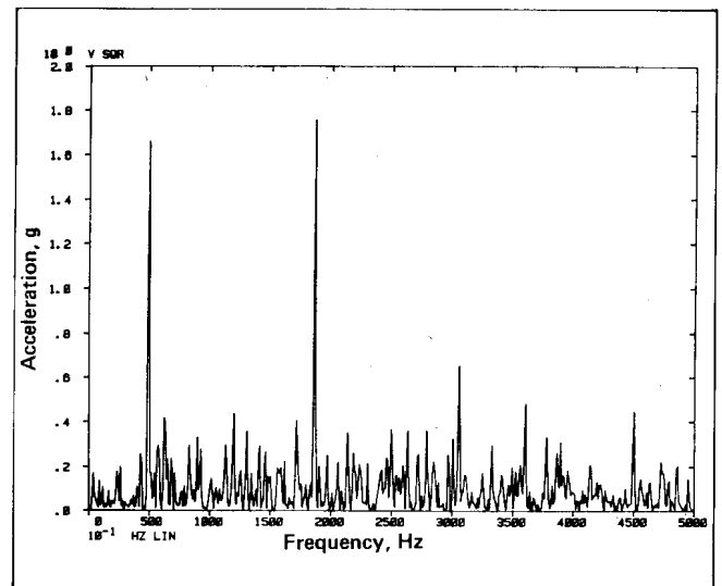
Figure 1. Vibration spectrum of an operating structure.
