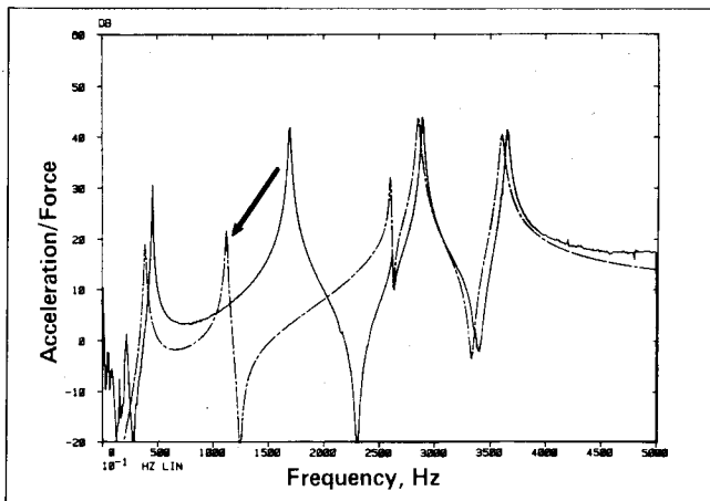
Figure 5. Reduction of objectionable structural response by shifting a problem mode to a lower frequency.
