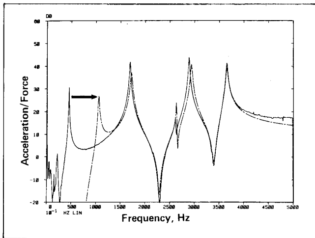
Figure 4. Reduction of objectionable structural response by shifting a problem mode to a higher frequency.
